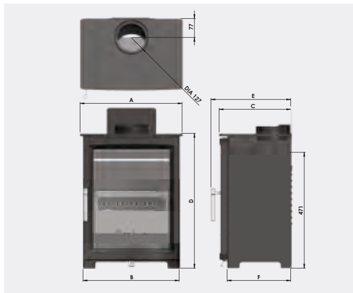
Woodtec 5 Stove
