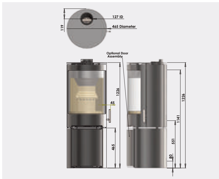
BPVR cylinder on high log store with door
