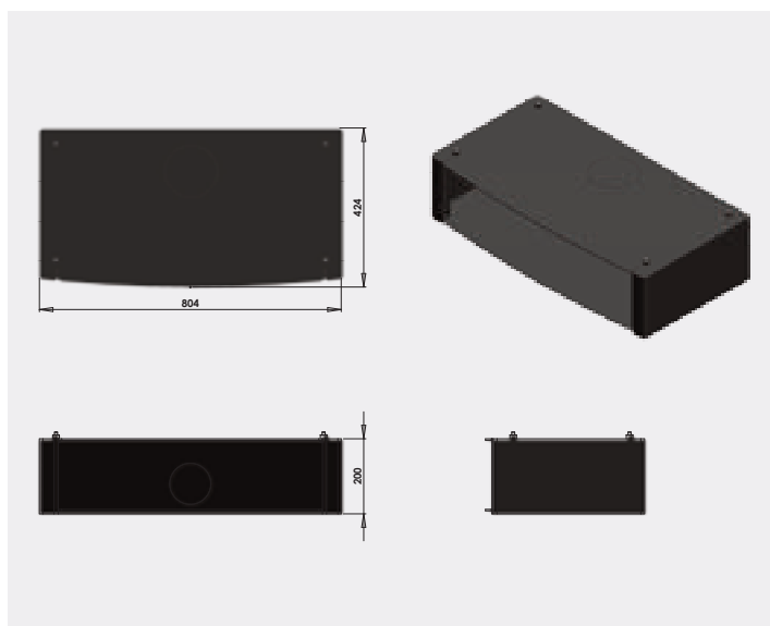
BPV8 Short Log Store
