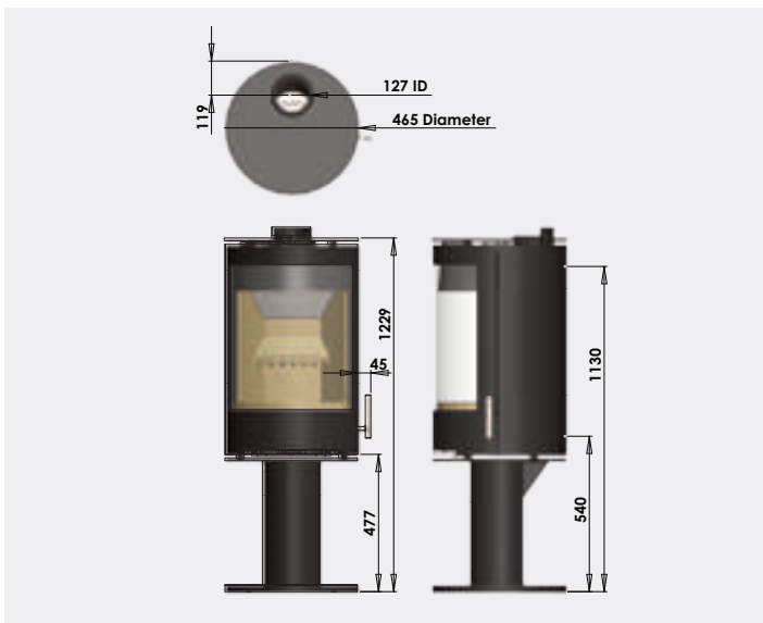
BPVR cylinder on high pedestal stand
