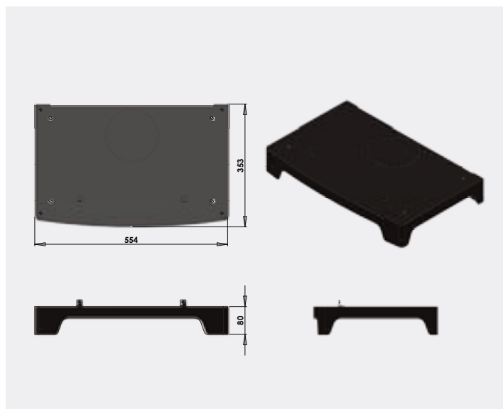
BPV5W Slimline Stand
